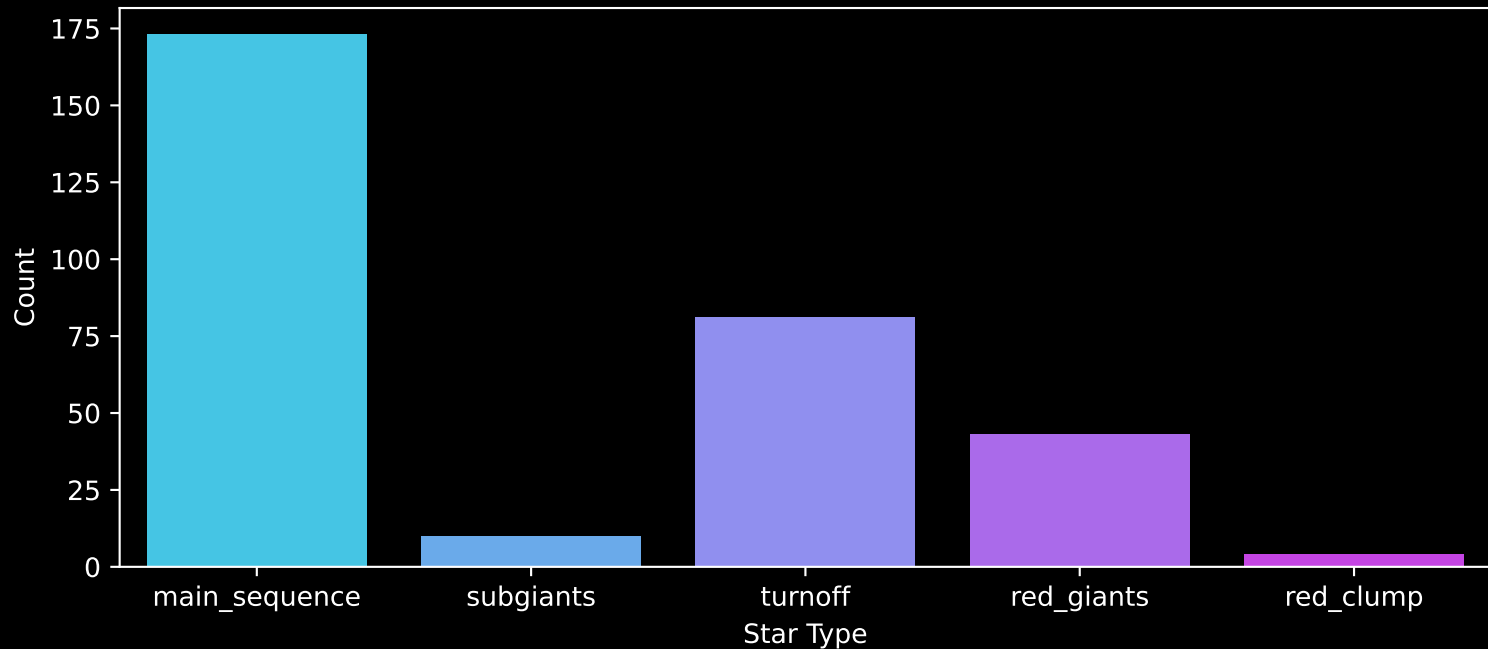
GALAH DR4 Field: [370] Count plot of Star Type
