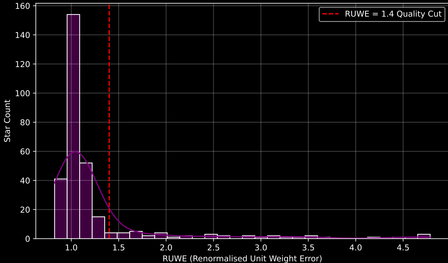
GALAH DR4 Field [370] RUWE Distribution (n= 305)
