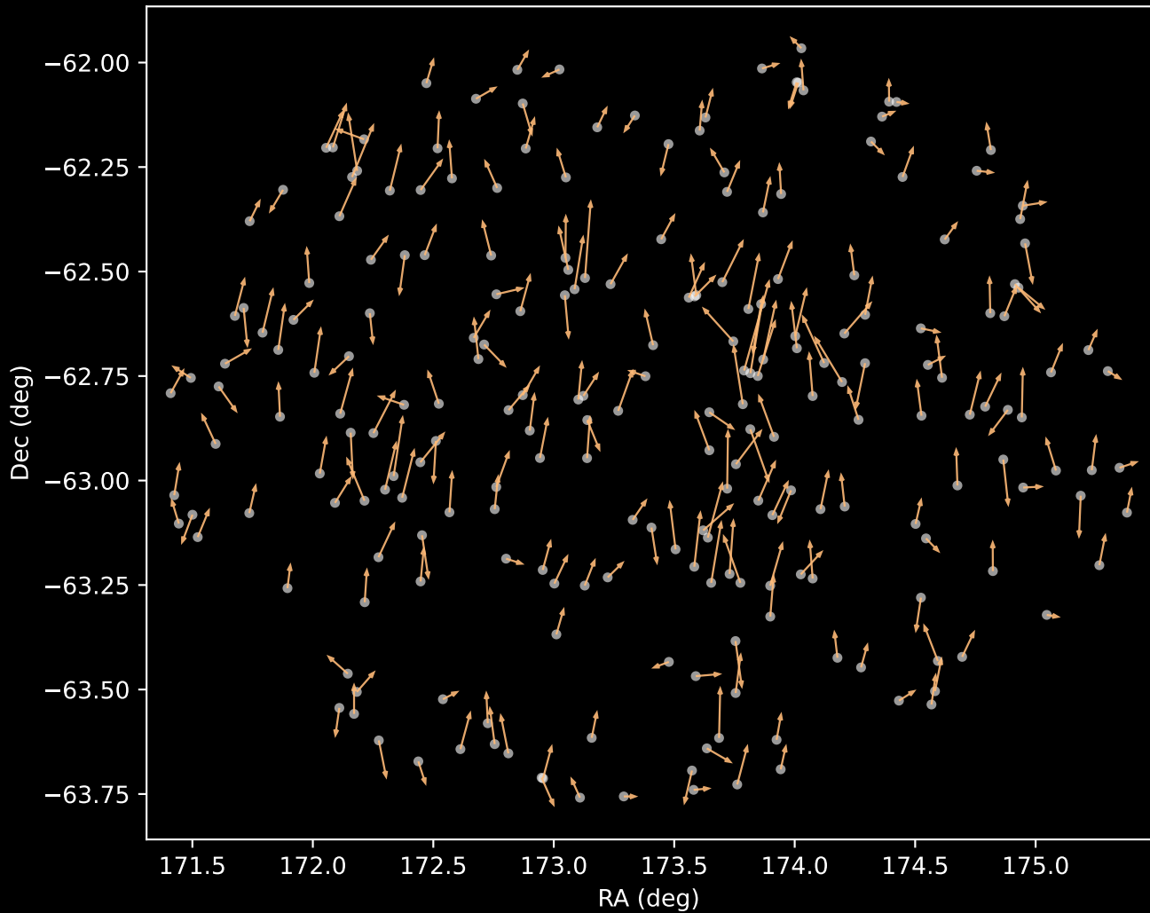
GALAH DR4 Cluster 3 Proper Motion Vectors (n=229)
