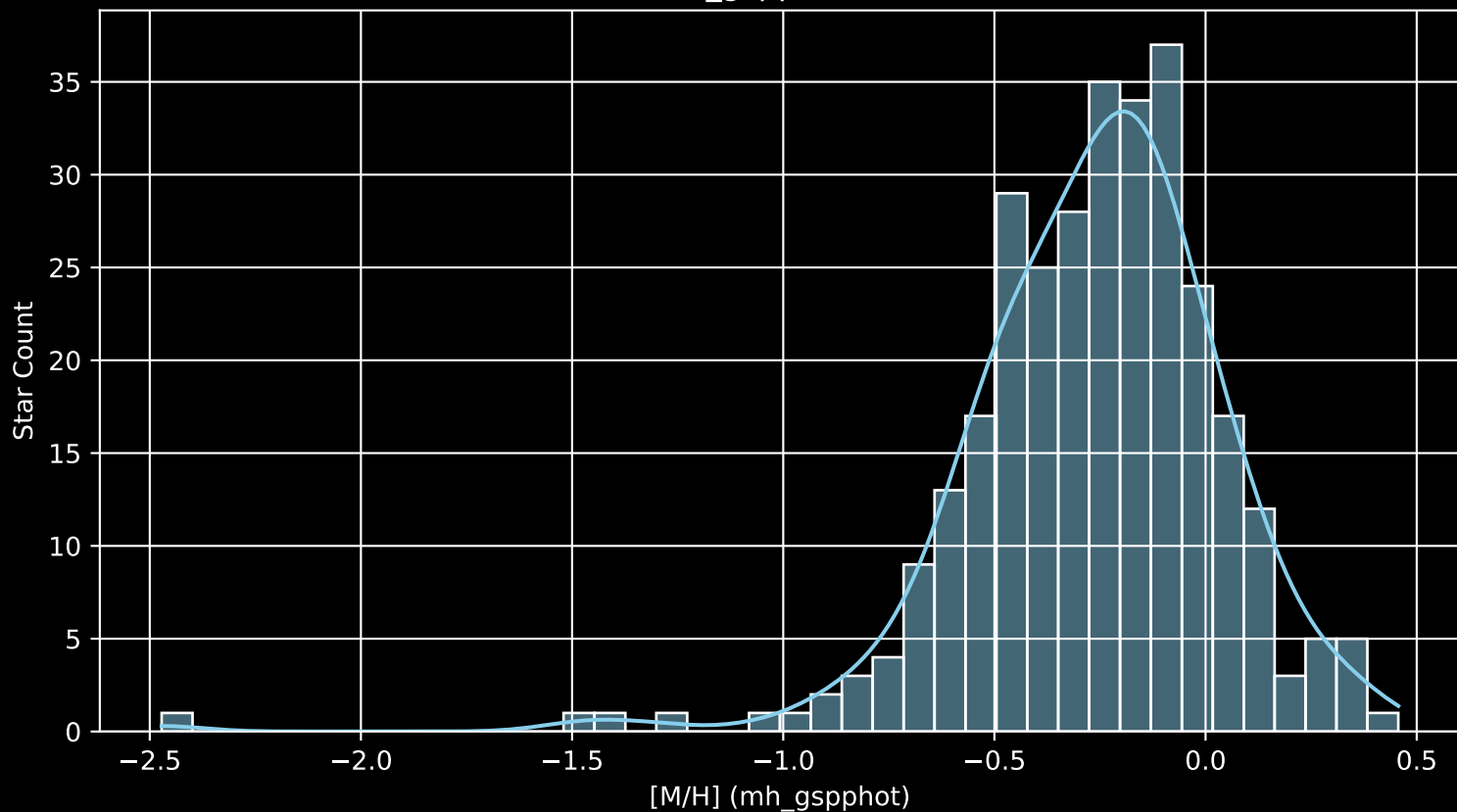
GALAH DR4 Field: [370] [M/H] (mh_gspphot) (n= 309)
